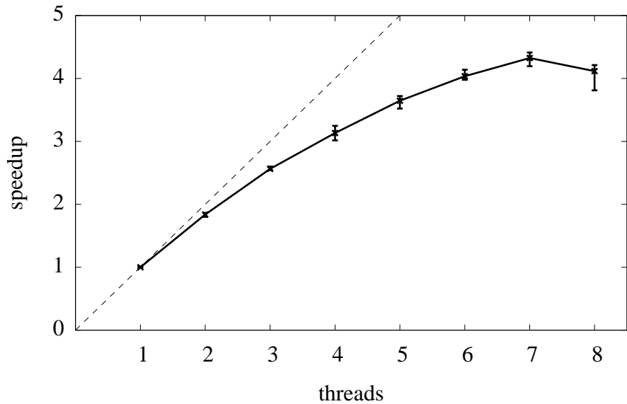
FFT3D on 2x Quad-core 3GHz Xenon
